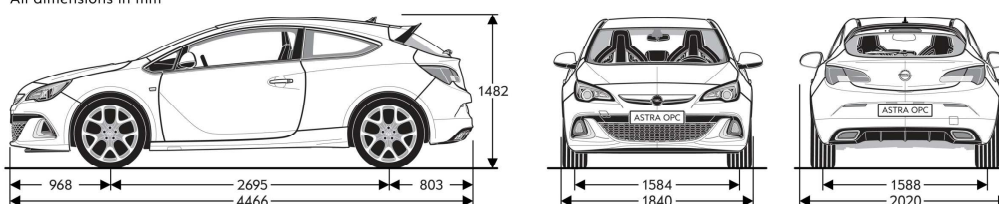
Astra OPC All dimensions in mm
